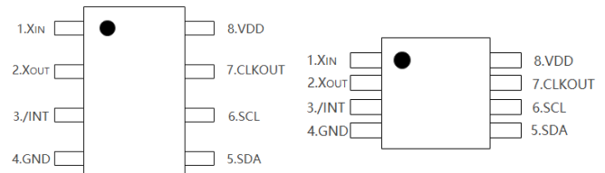
YSN8563TS (SOP-8)
