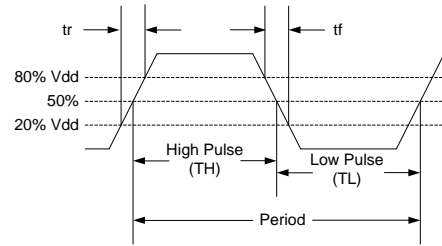
Figure 3. Waveform [8]
