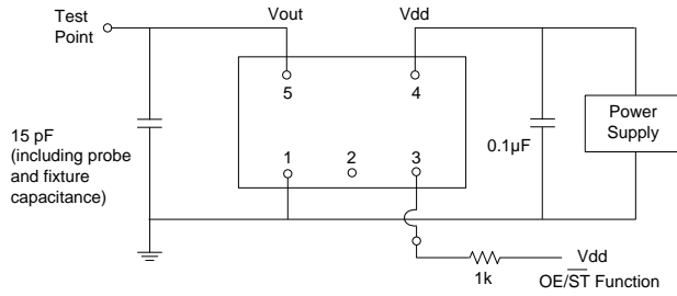
Figure 2. Test Circuit [6]
